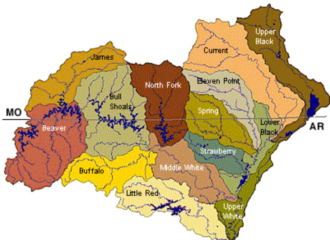
Watersheds of the White River Basin
